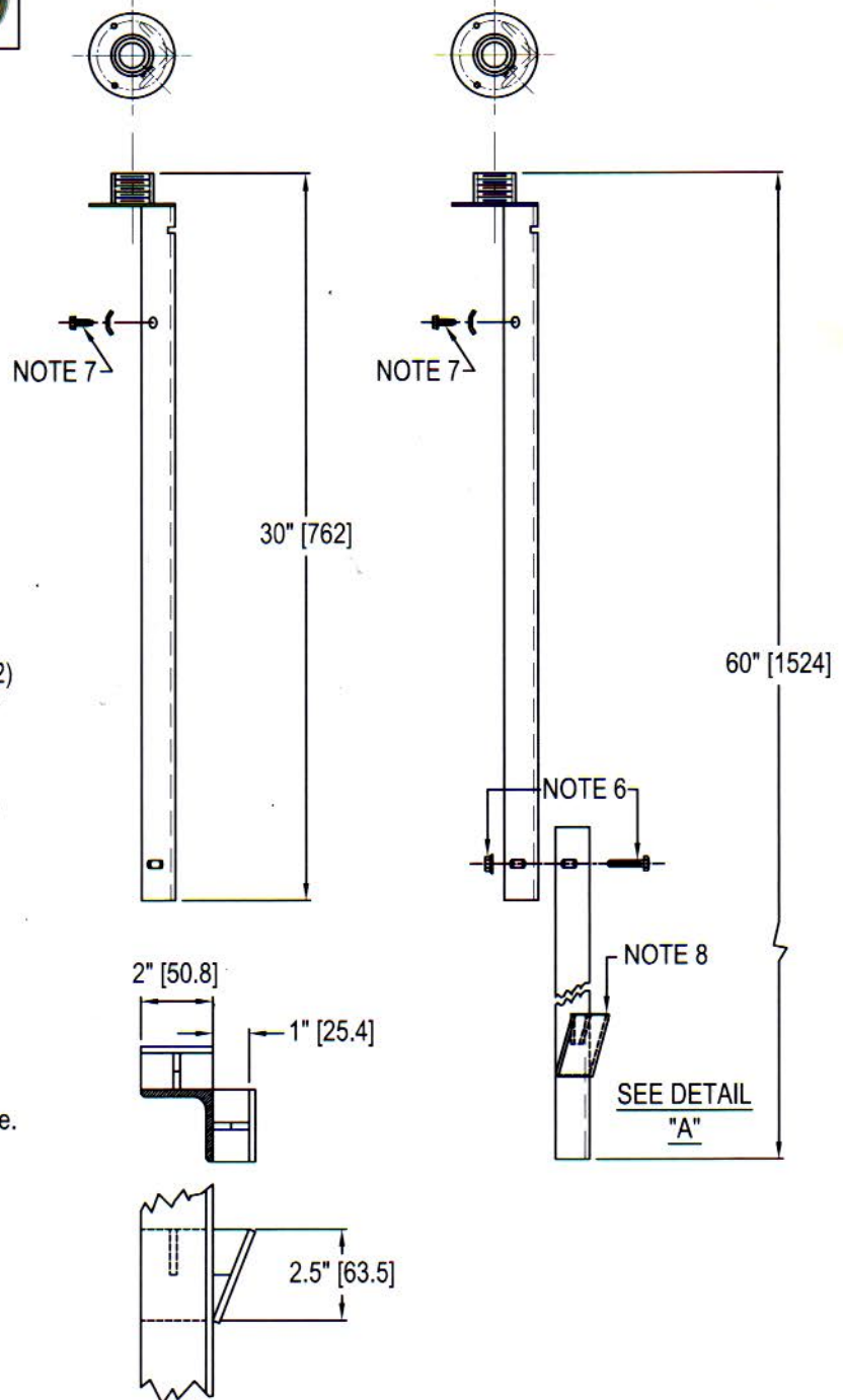
DETAIL "A"
